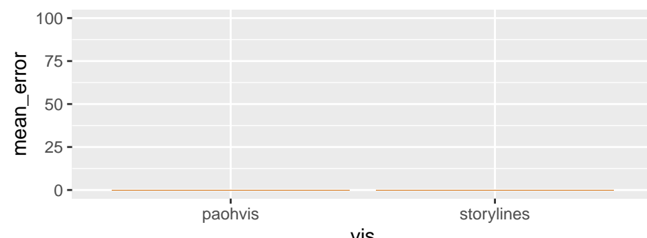
Error Rate
